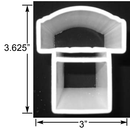
Breadloaf Rail
